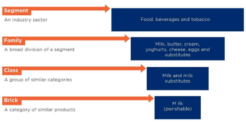
Figure 2.1: GPC layers
